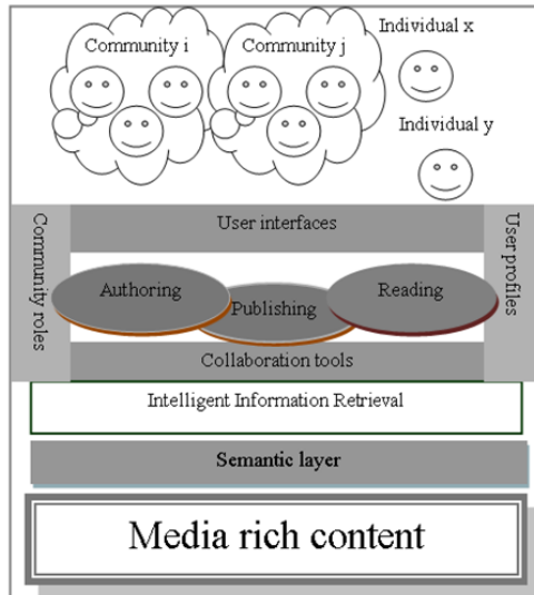
Fig. 1. SmartBook architecture.
